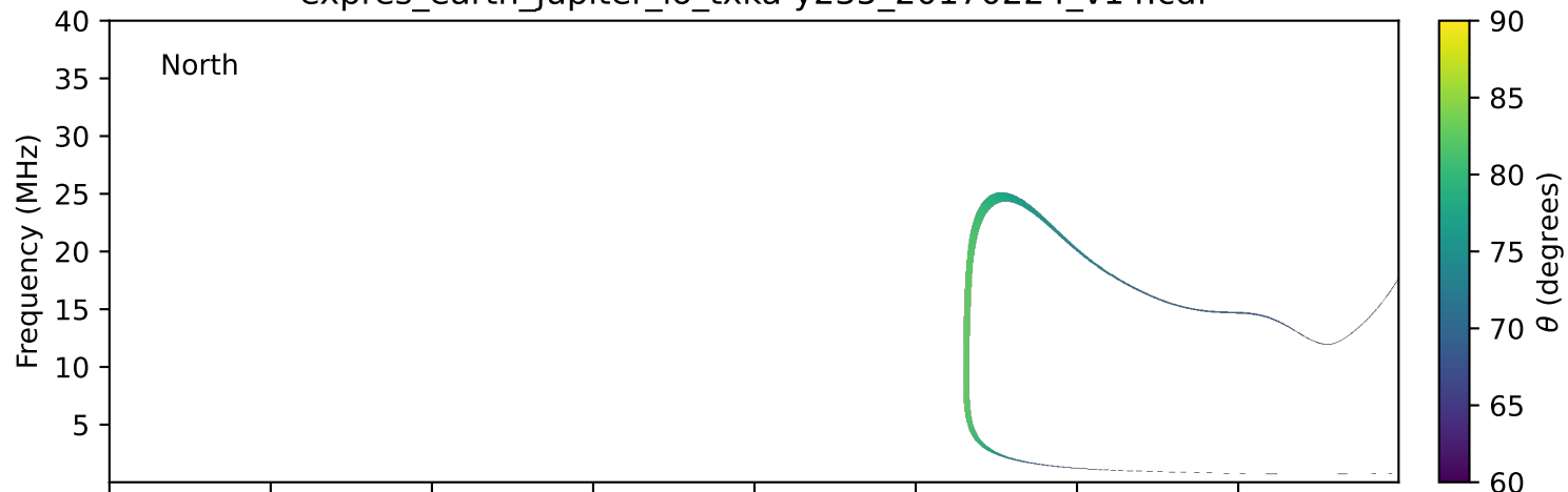
expres_earth_jupiter_io_txka-y235_20170224_v14.cdf
