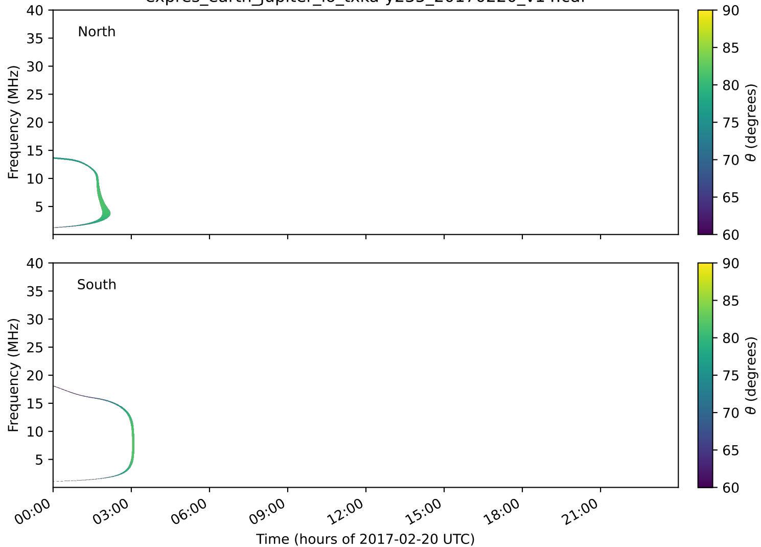
expres_earth_jupiter_io_txka-y235_20170220_v14.cdf
