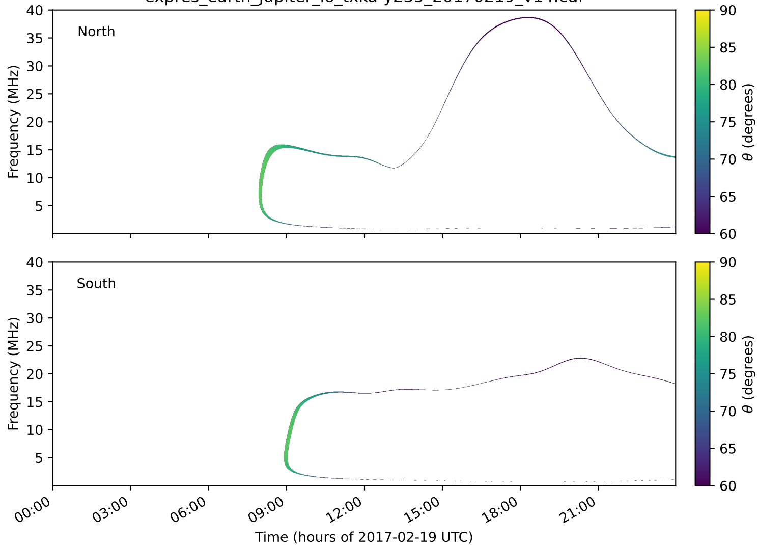
expres_earth_jupiter_io_txka-y235_20170219_v14.cdf
