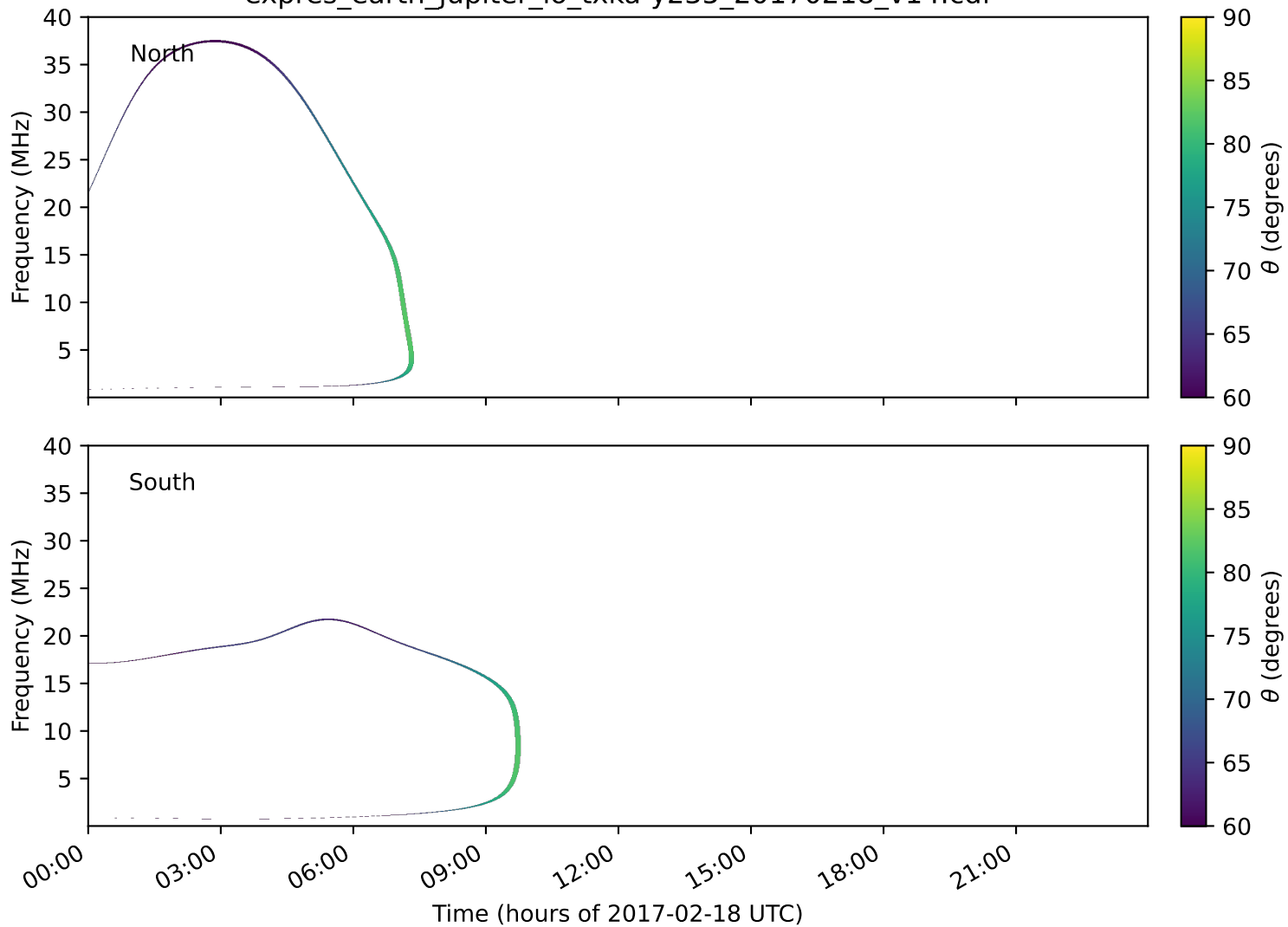
expres_earth_jupiter_io_txka-y235_20170218_v14.cdf
