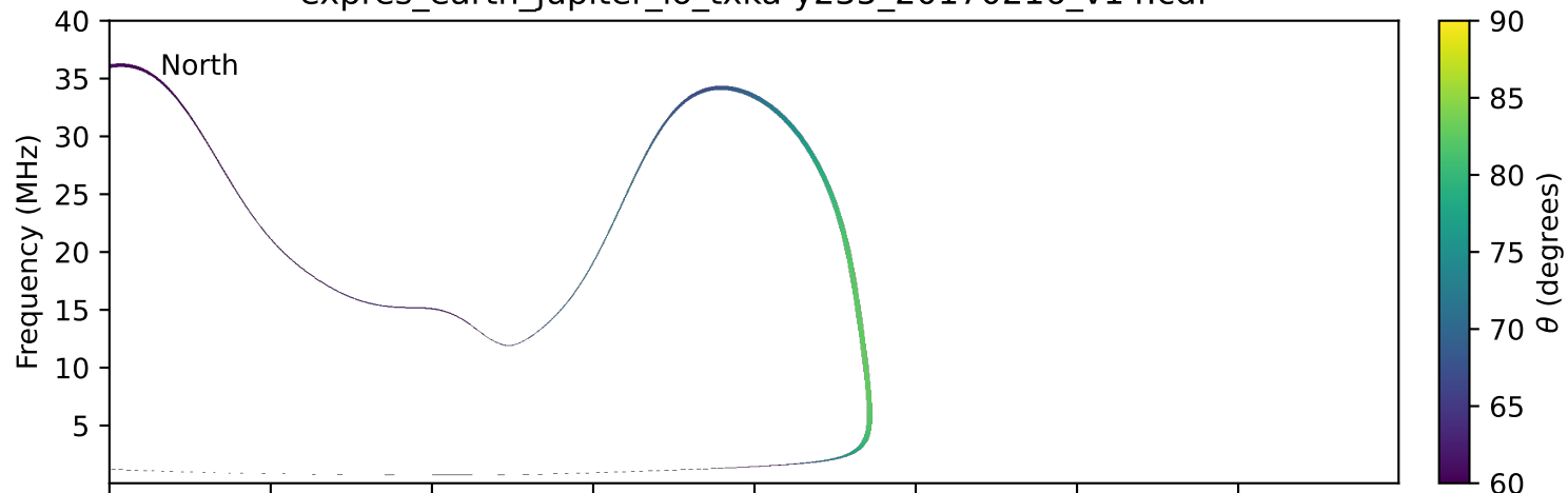
expres_earth_jupiter_io_txka-y235_20170216_v14.cdf
