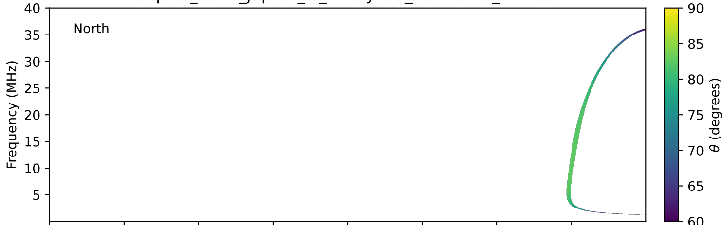
expres_earth_jupiter_io_txka-y235_20170215_v14.cdf
