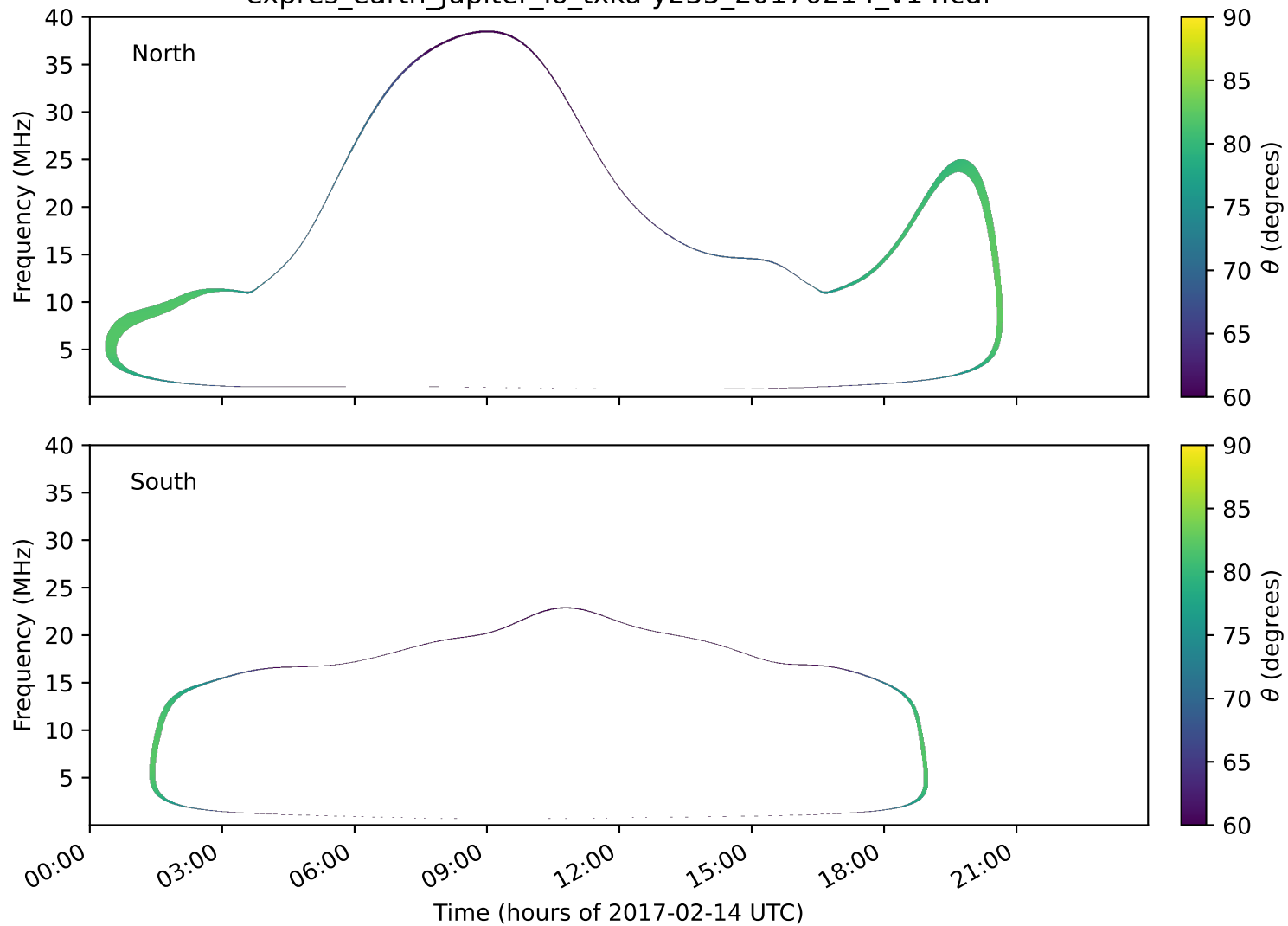
expres_earth_jupiter_io_txka-y235_20170214_v14.cdf
