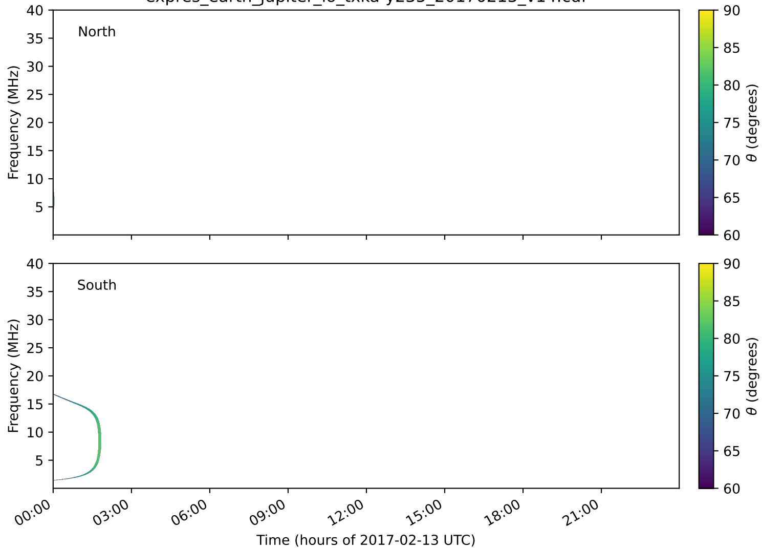
expres_earth_jupiter_io_txka-y235_20170213_v14.cdf
