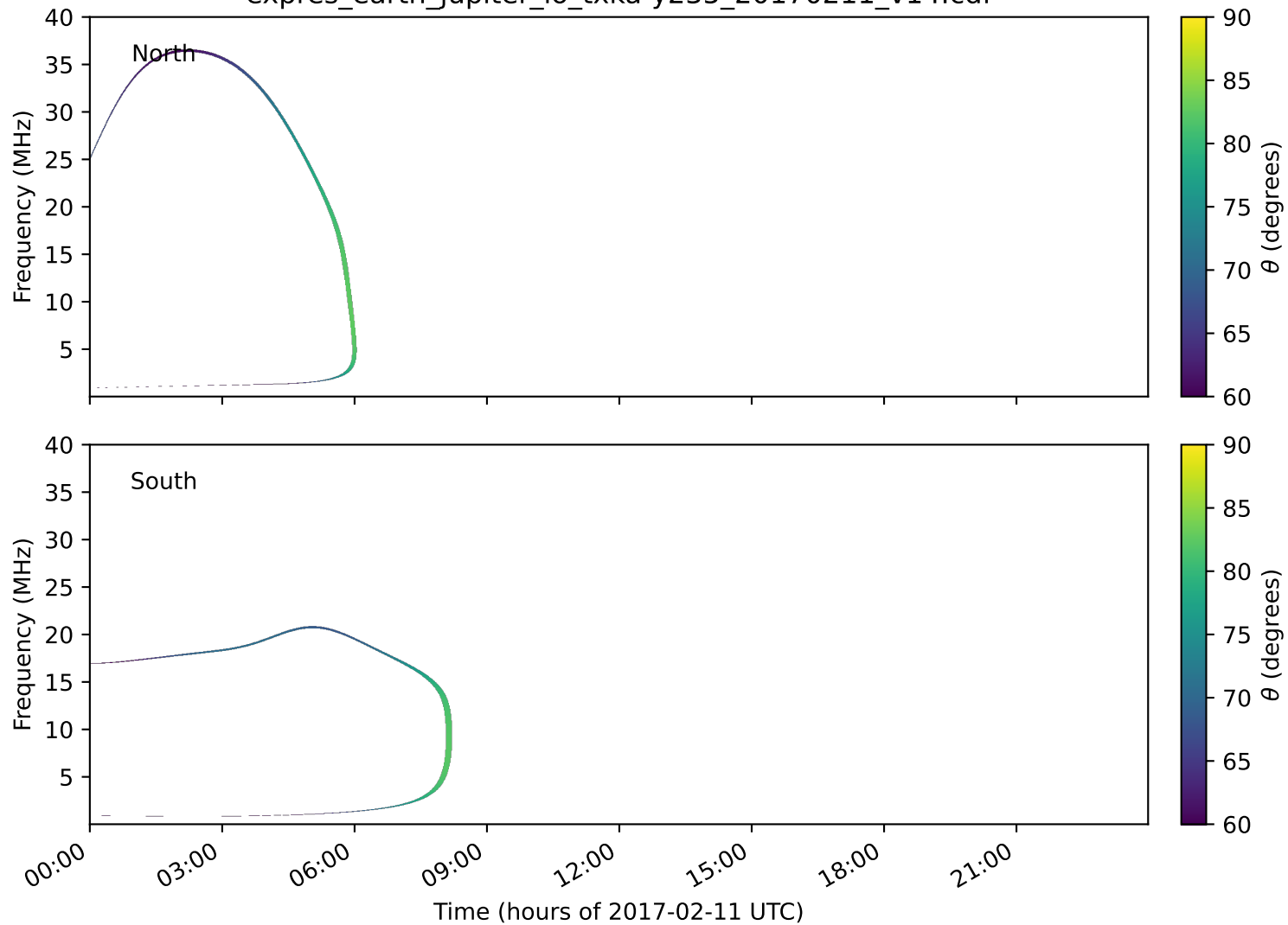
expres_earth_jupiter_io_txka-y235_20170211_v14.cdf
