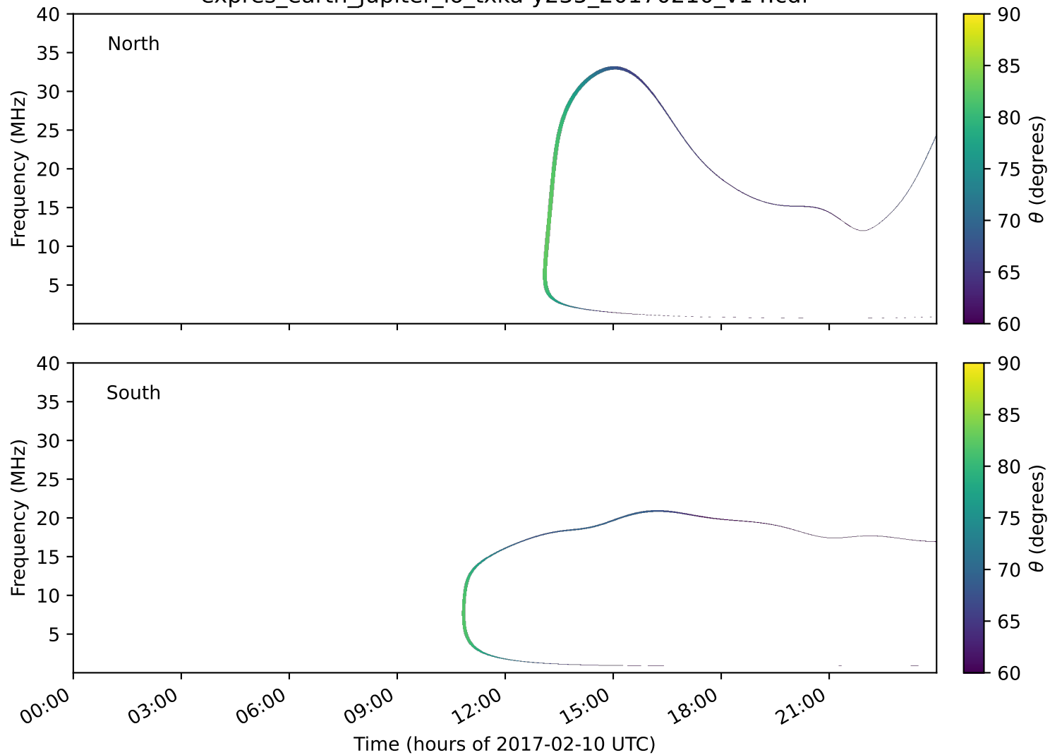
expres_earth_jupiter_io_txka-y235_20170210_v14.cdf
