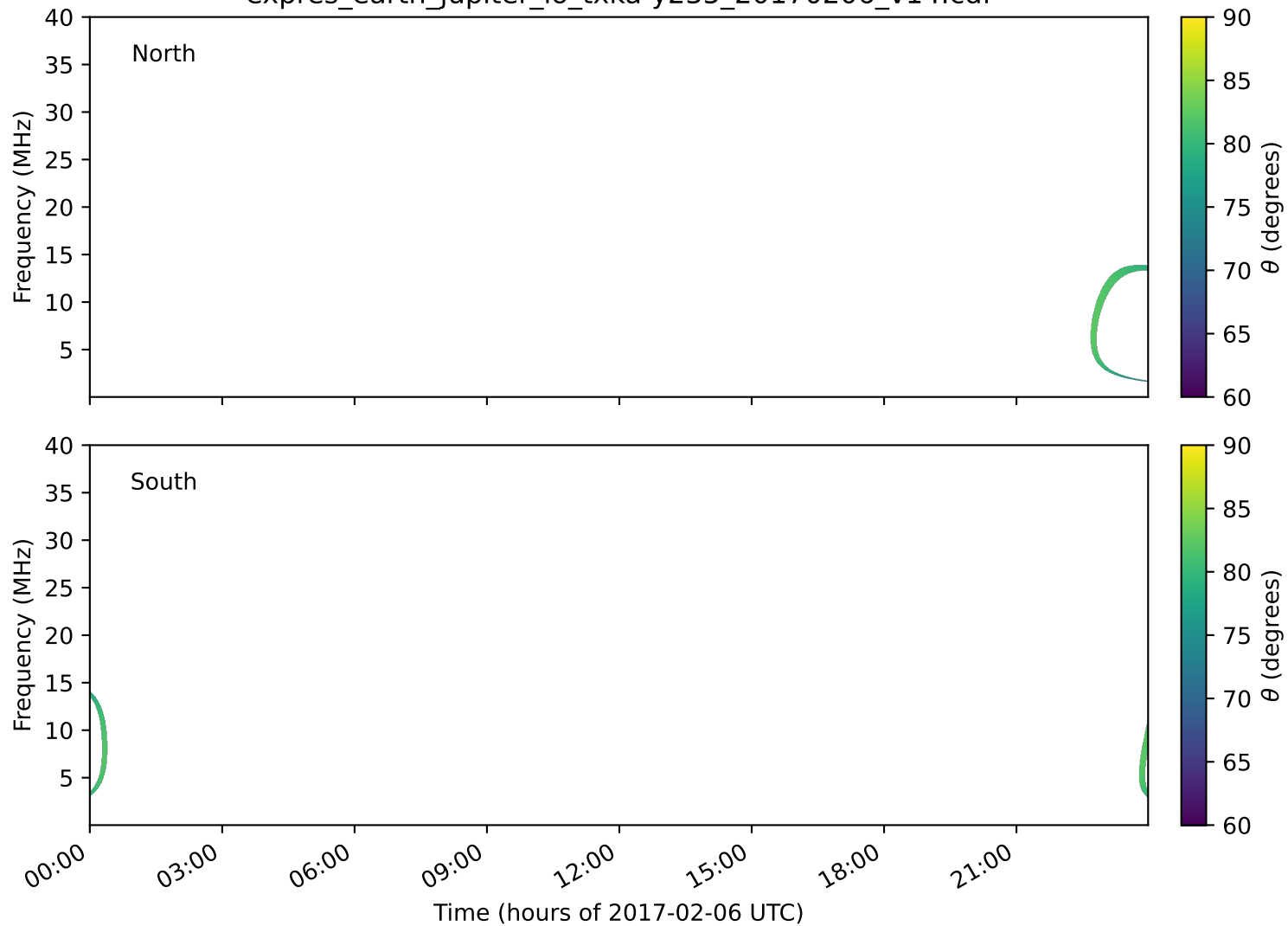
expres_earth_jupiter_io_txka-y235_20170206_v14.cdf
