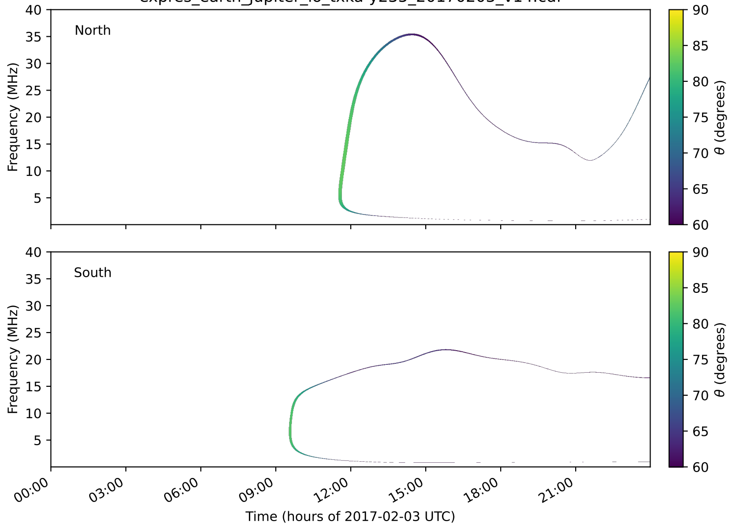
expres_earth_jupiter_io_txka-y235_20170203_v14.cdf
