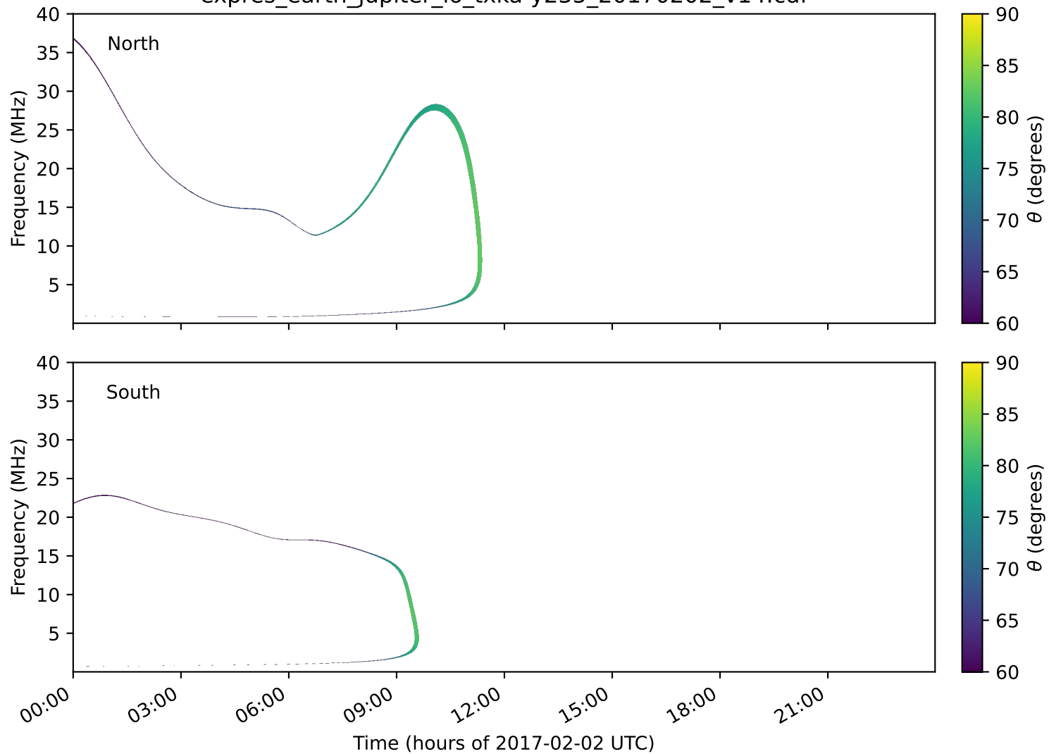
expres_earth_jupiter_io_txka-y235_20170202_v14.cdf
