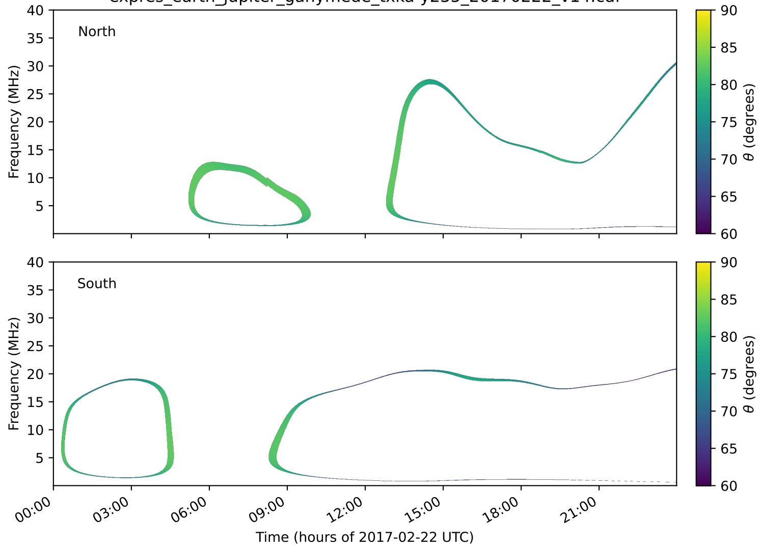
expres_earth_jupiter_ganymede_txka-y235_20170222_v14.cdf
