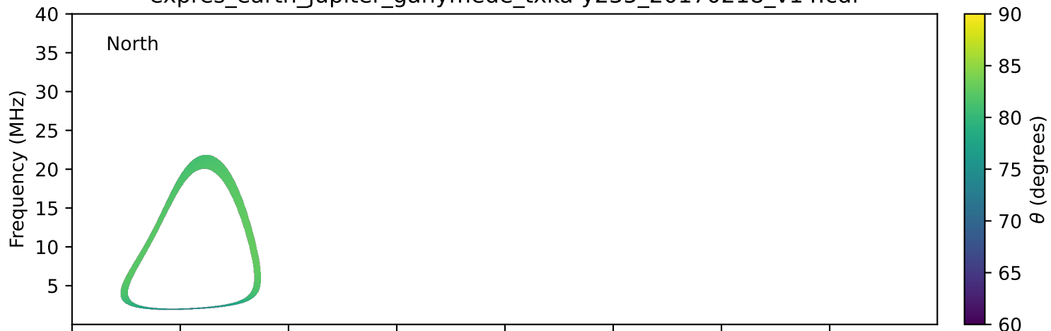
expres_earth_jupiter_ganymede_txka-y235_20170218_v14.cdf
