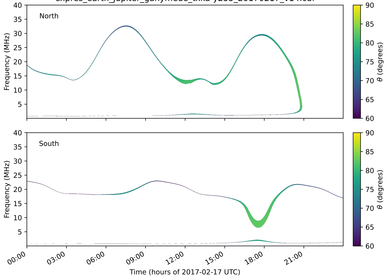
expres_earth_jupiter_ganymede_txka-y235_20170217_v14.cdf
