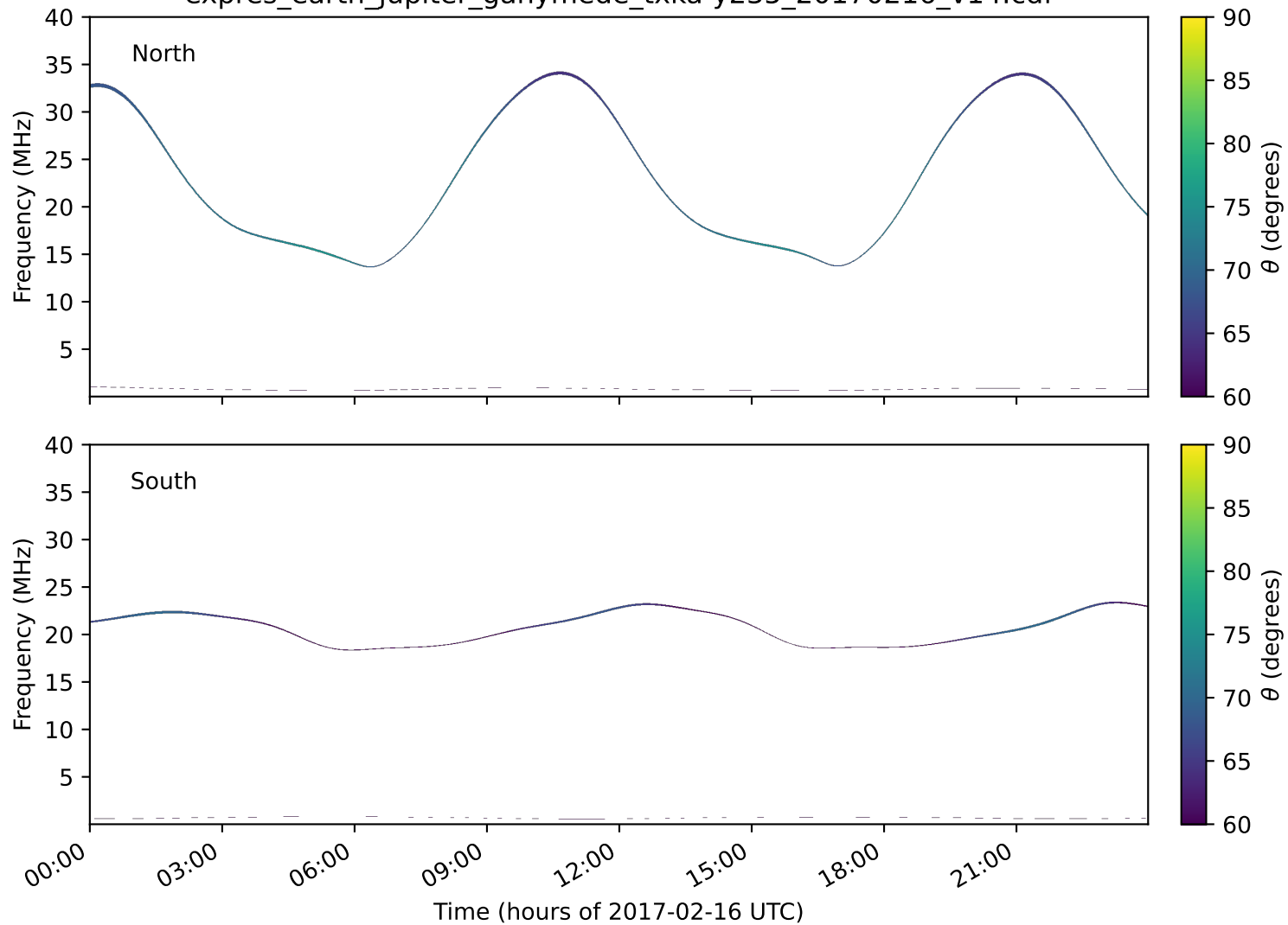
expres_earth_jupiter_ganymede_txka-y235_20170216_v14.cdf
