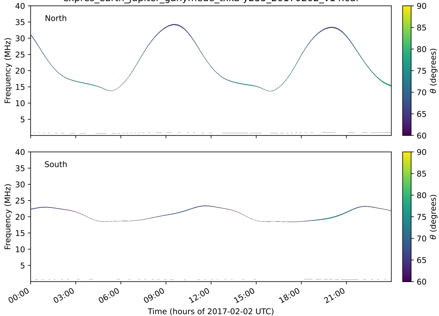
expres_earth_jupiter_ganymede_txka-y235_20170202_v14.cdf
