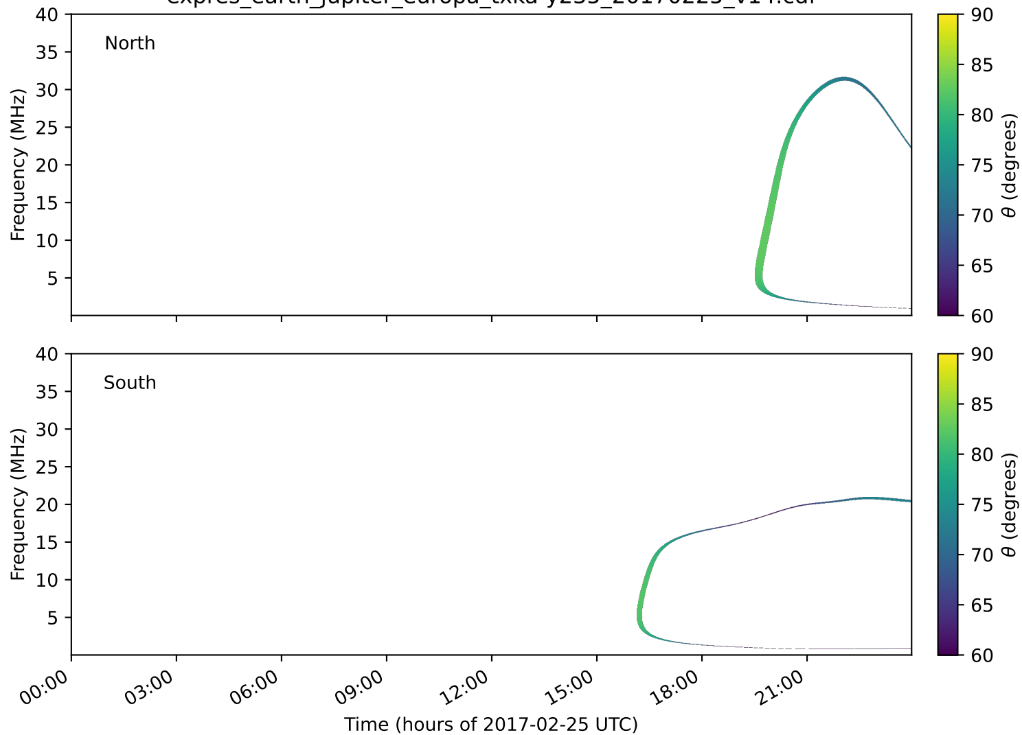
expres_earth_jupiter_europa_txka-y235_20170225_v14.cdf
