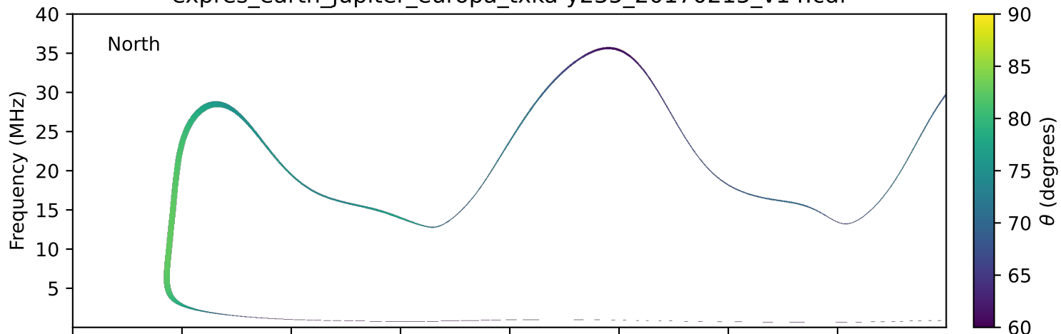
expres_earth_jupiter_europa_txka-y235_20170215_v14.cdf
