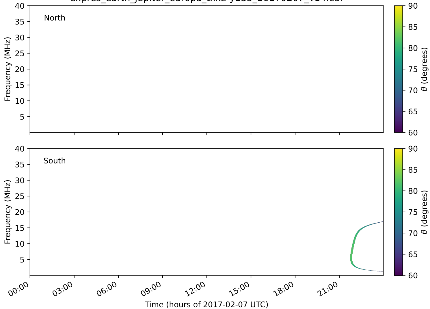
expres_earth_jupiter_europa_txka-y235_20170207_v14.cdf
