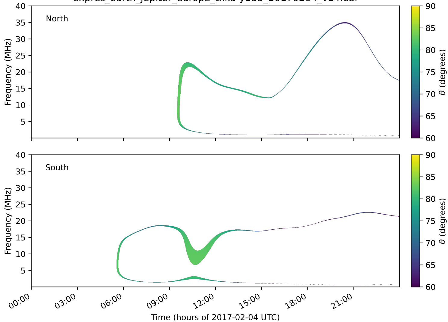
expres_earth_jupiter_europa_txka-y235_20170204_v14.cdf
