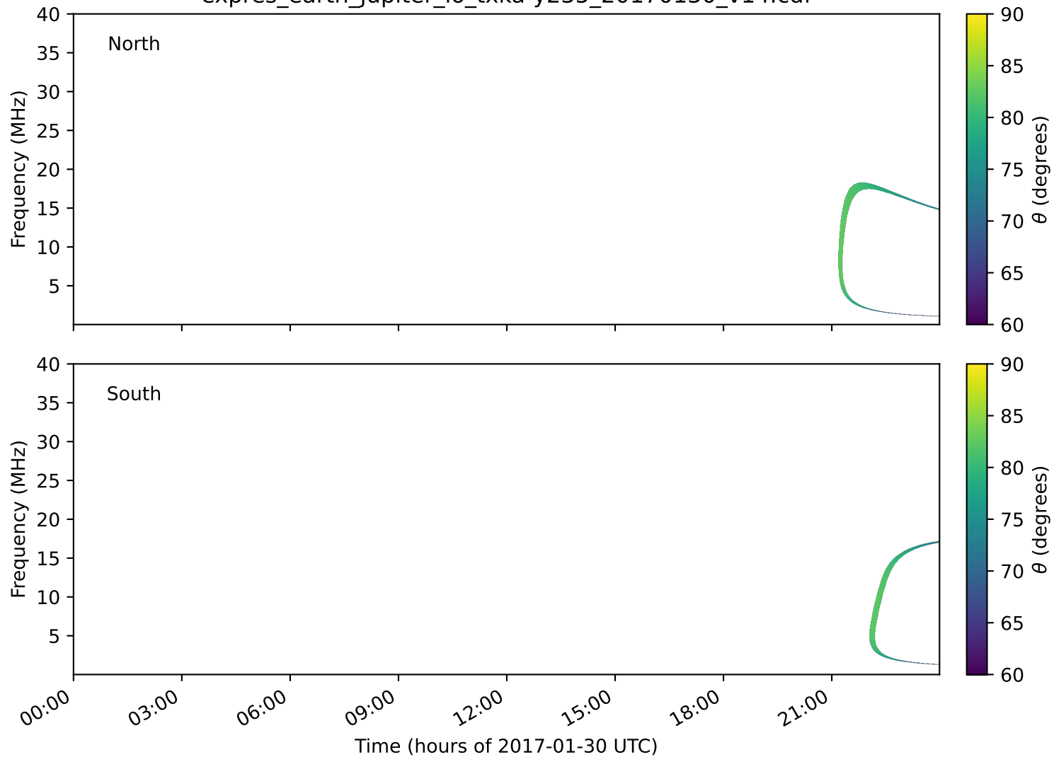
expres_earth_jupiter_io_txka-y235_20170130_v14.cdf
