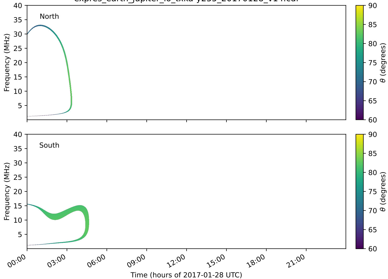
expres_earth_jupiter_io_txka-y235_20170128_v14.cdf
