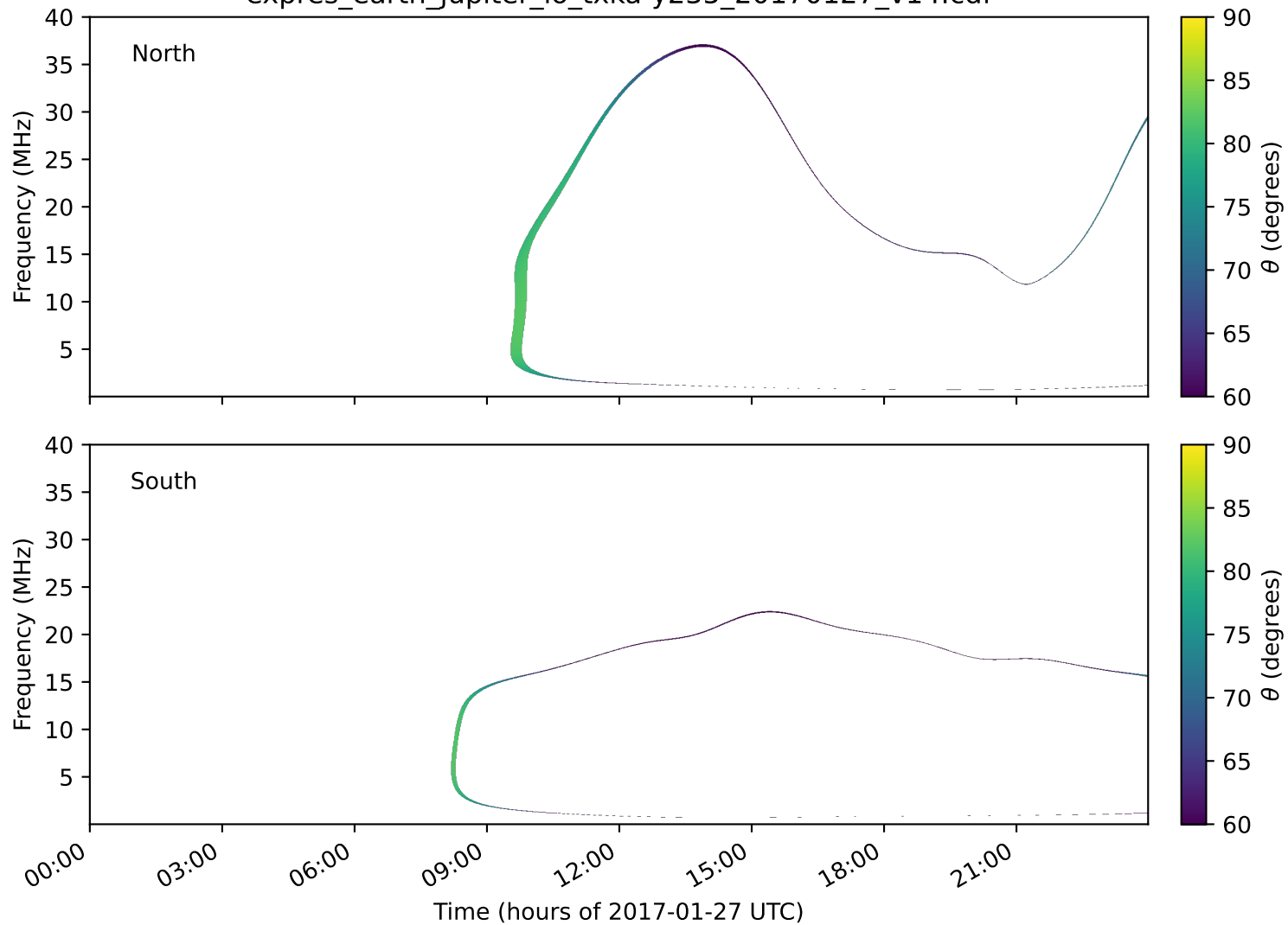
expres_earth_jupiter_io_txka-y235_20170127_v14.cdf
