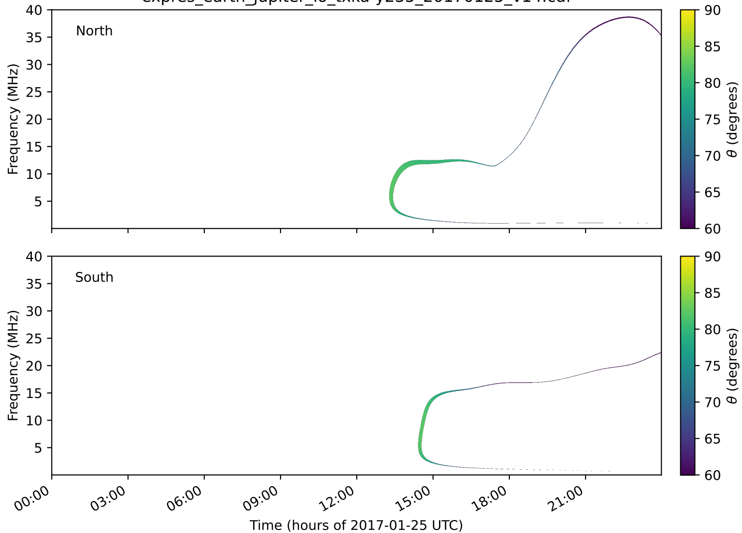
expres_earth_jupiter_io_txka-y235_20170125_v14.cdf
