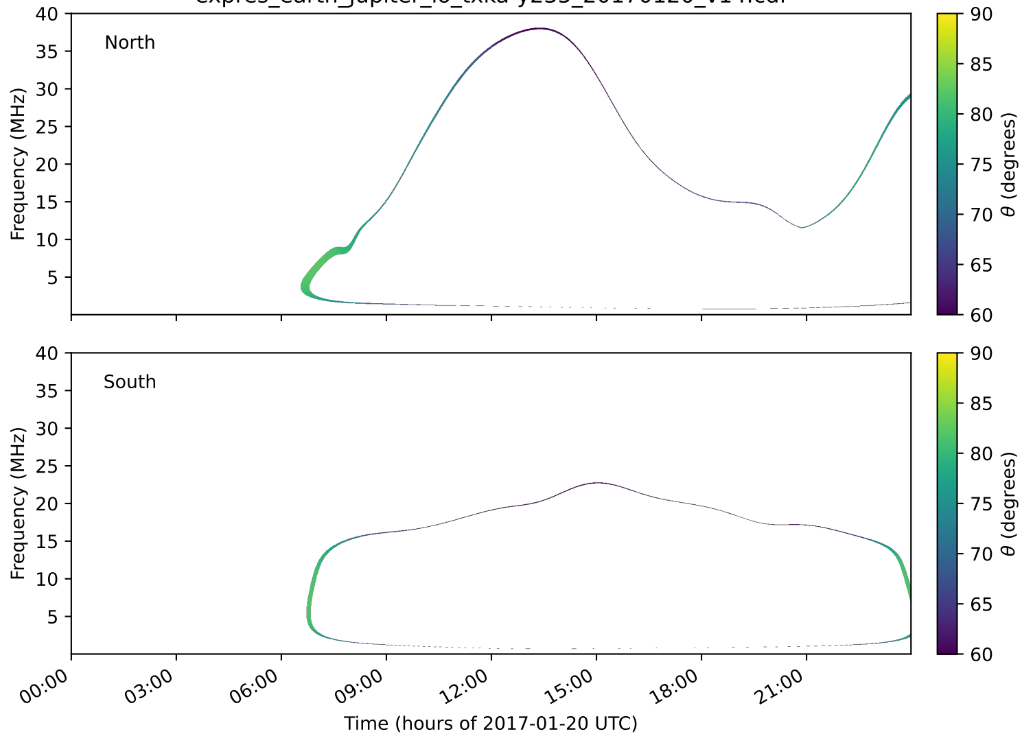
expres_earth_jupiter_io_txka-y235_20170120_v14.cdf
