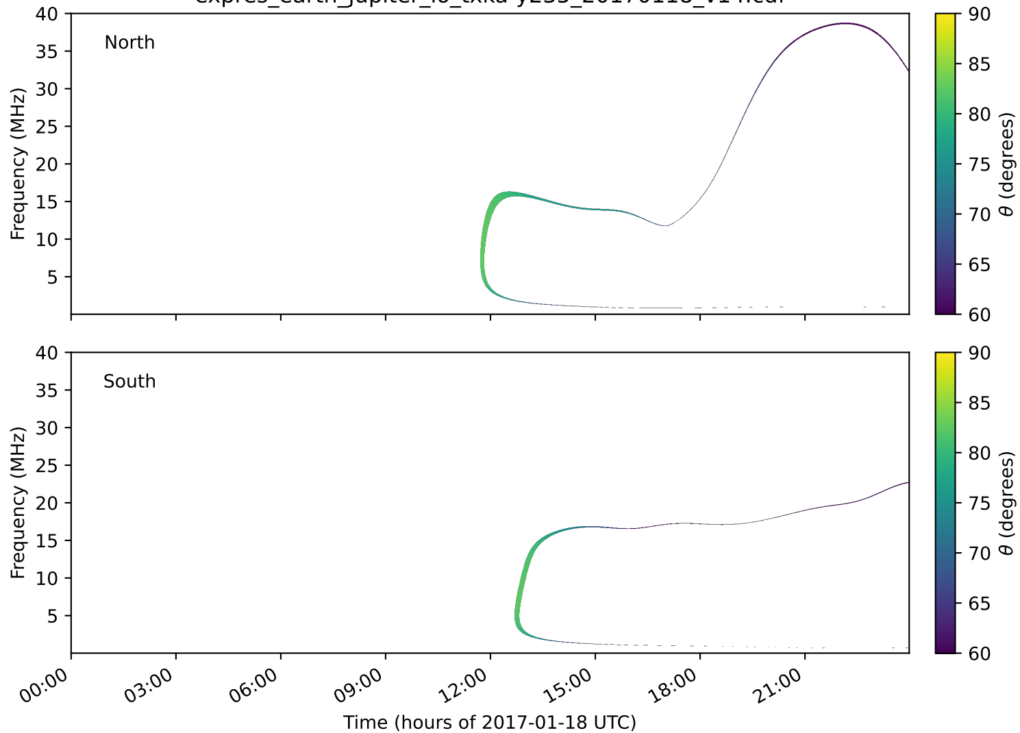
expres_earth_jupiter_io_txka-y235_20170118_v14.cdf
