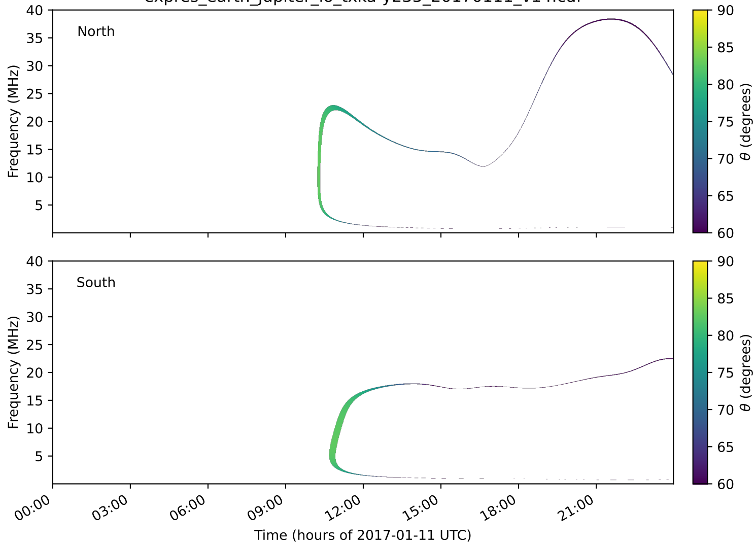
expres_earth_jupiter_io_txka-y235_20170111_v14.cdf
