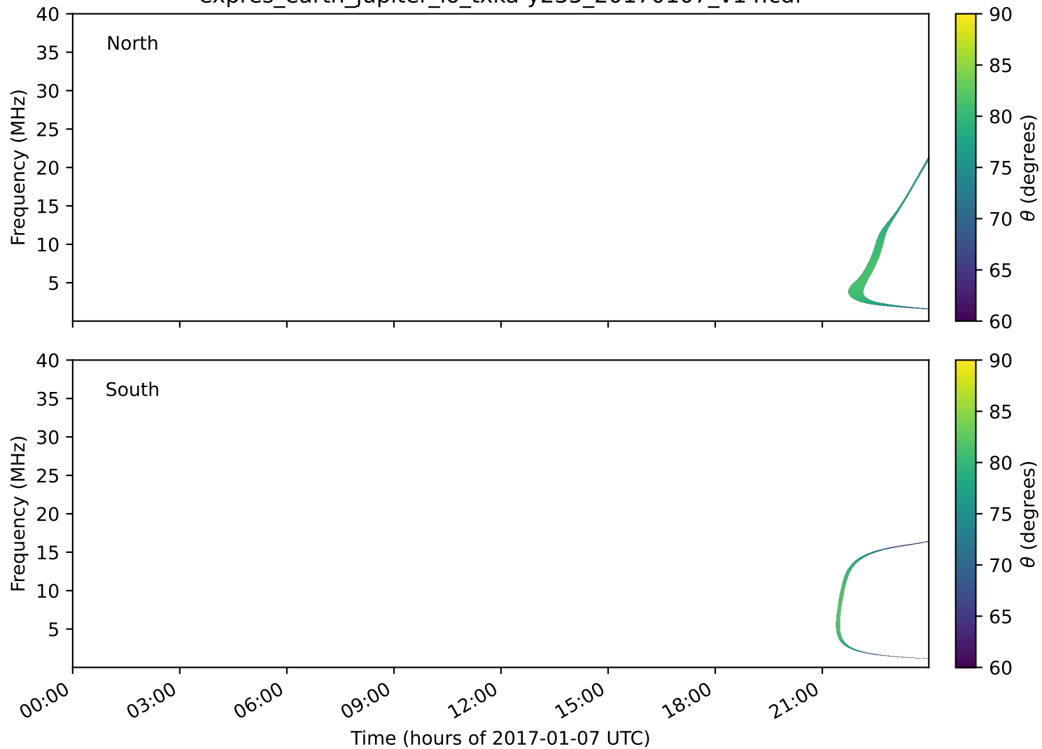
expres_earth_jupiter_io_txka-y235_20170107_v14.cdf
