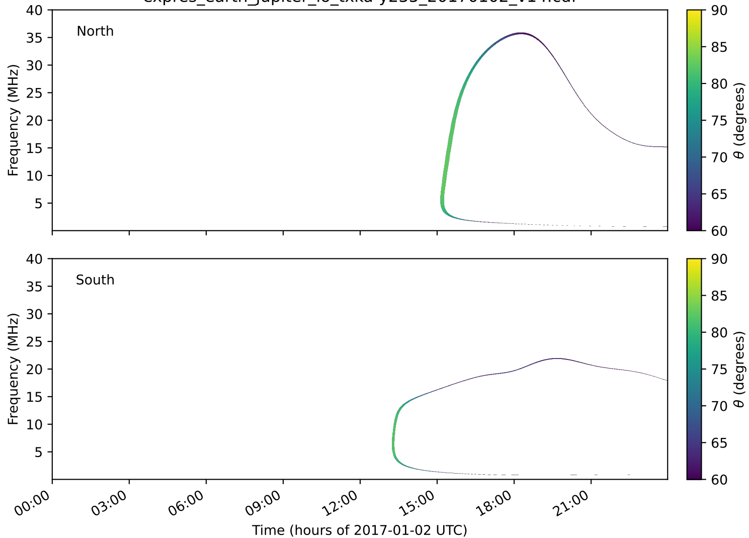
expres_earth_jupiter_io_txka-y235_20170102_v14.cdf
