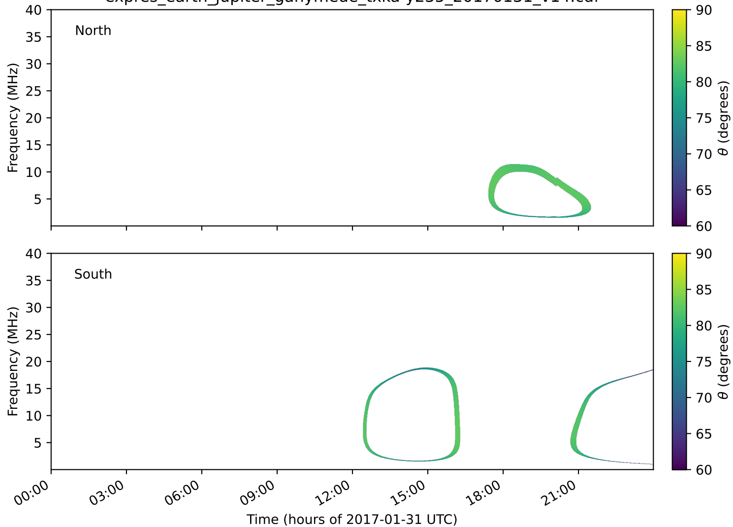
expres_earth_jupiter_ganymede_txka-y235_20170131_v14.cdf
