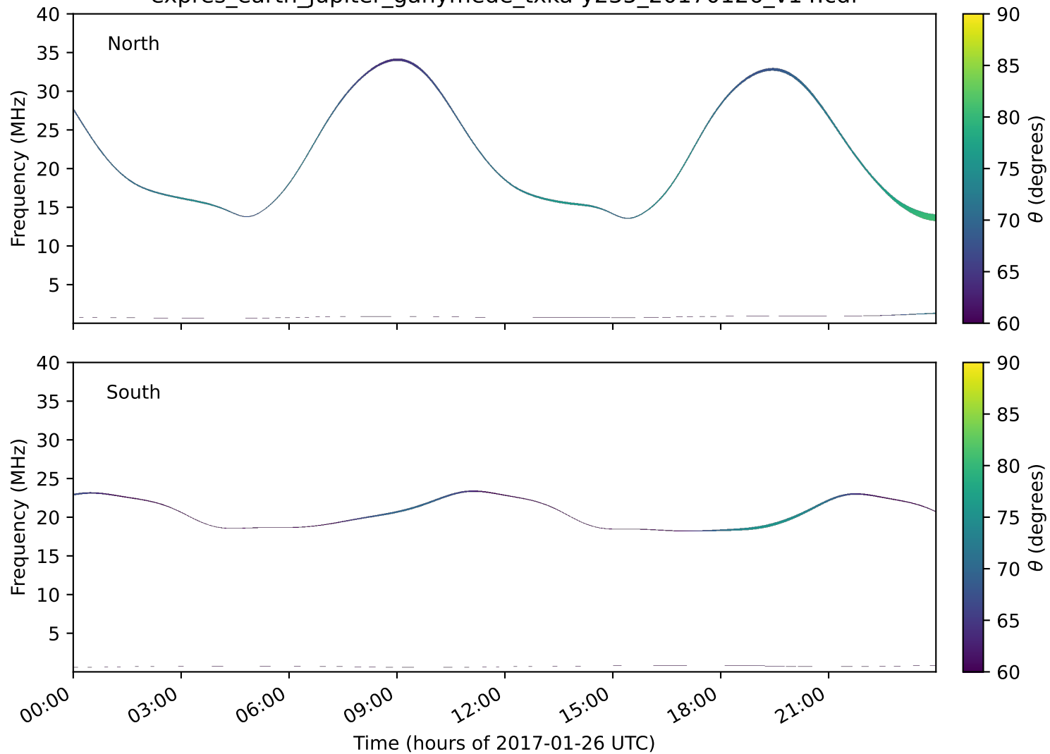
expres_earth_jupiter_ganymede_txka-y235_20170126_v14.cdf
