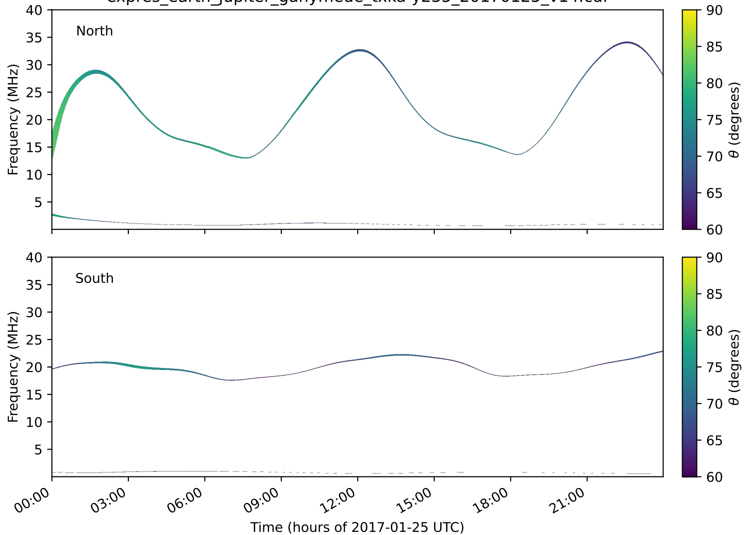
expres_earth_jupiter_ganymede_txka-y235_20170125_v14.cdf
