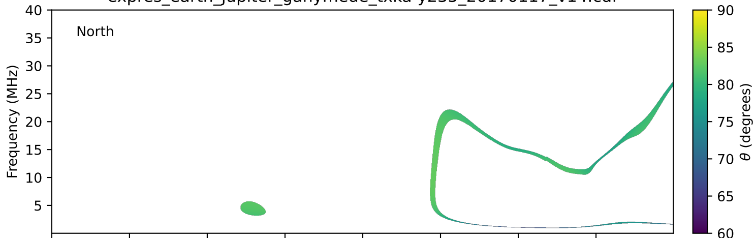
expres_earth_jupiter_ganymede_txka-y235_20170117_v14.cdf
