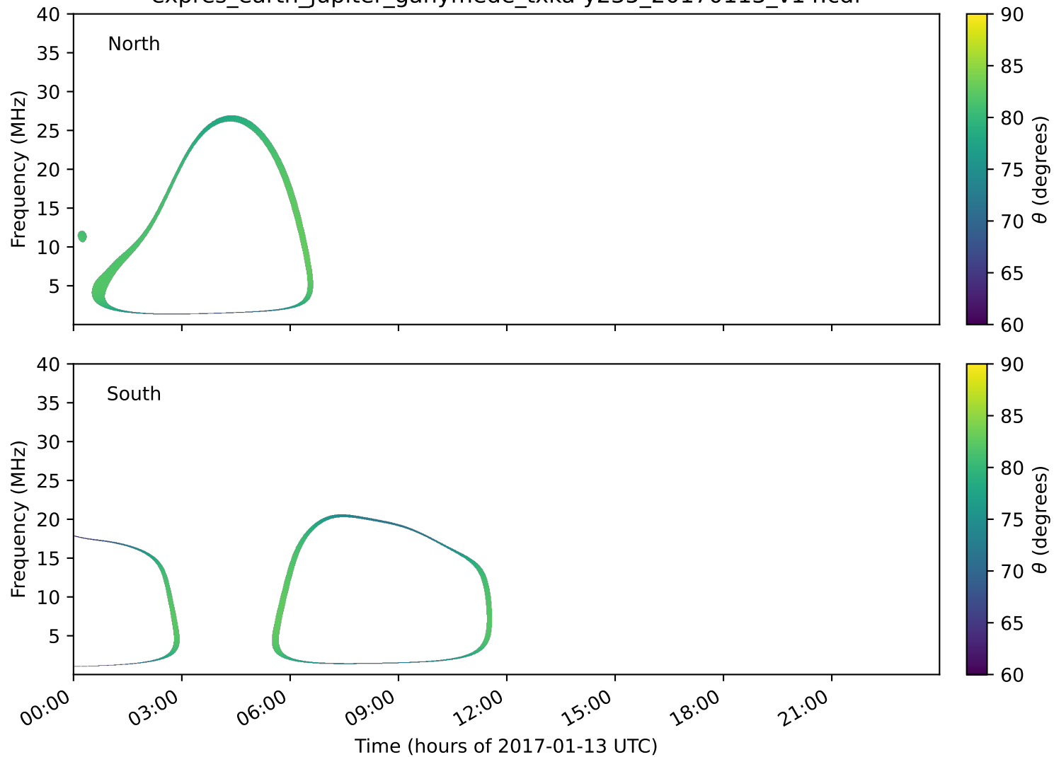
expres_earth_jupiter_ganymede_txka-y235_20170113_v14.cdf
