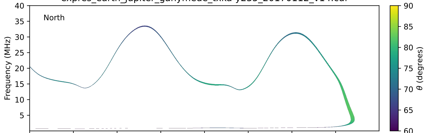
expres_earth_jupiter_ganymede_txka-y235_20170112_v14.cdf
