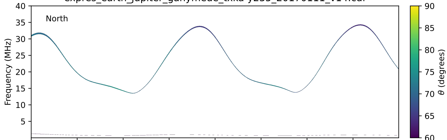
expres_earth_jupiter_ganymede_txka-y235_20170111_v14.cdf
