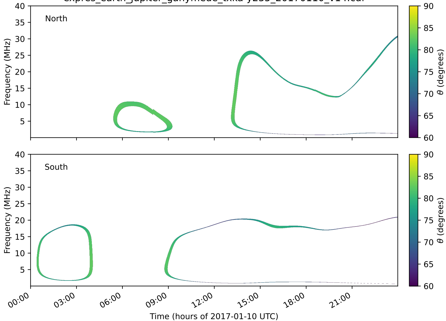
expres_earth_jupiter_ganymede_txka-y235_20170110_v14.cdf
