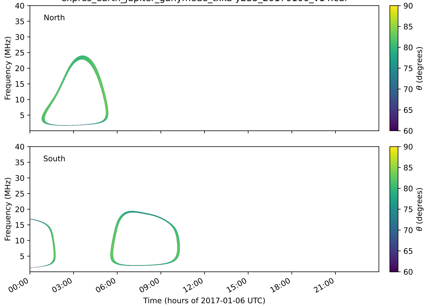
expres_earth_jupiter_ganymede_txka-y235_20170106_v14.cdf
