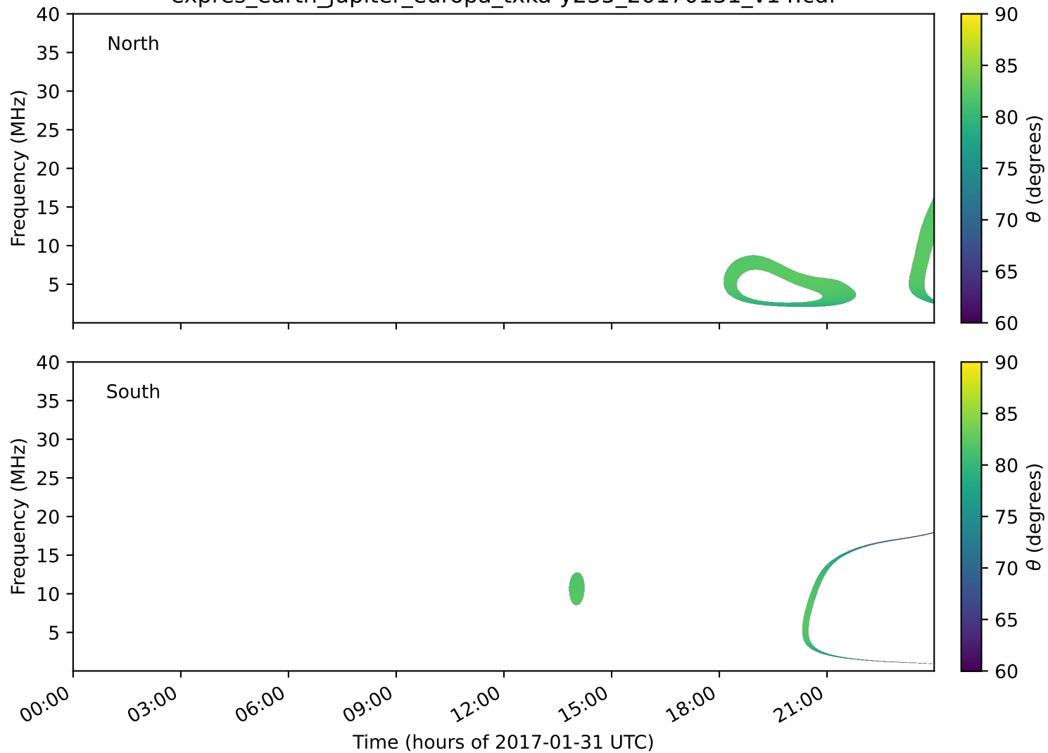
expres_earth_jupiter_europa_txka-y235_20170131_v14.cdf
