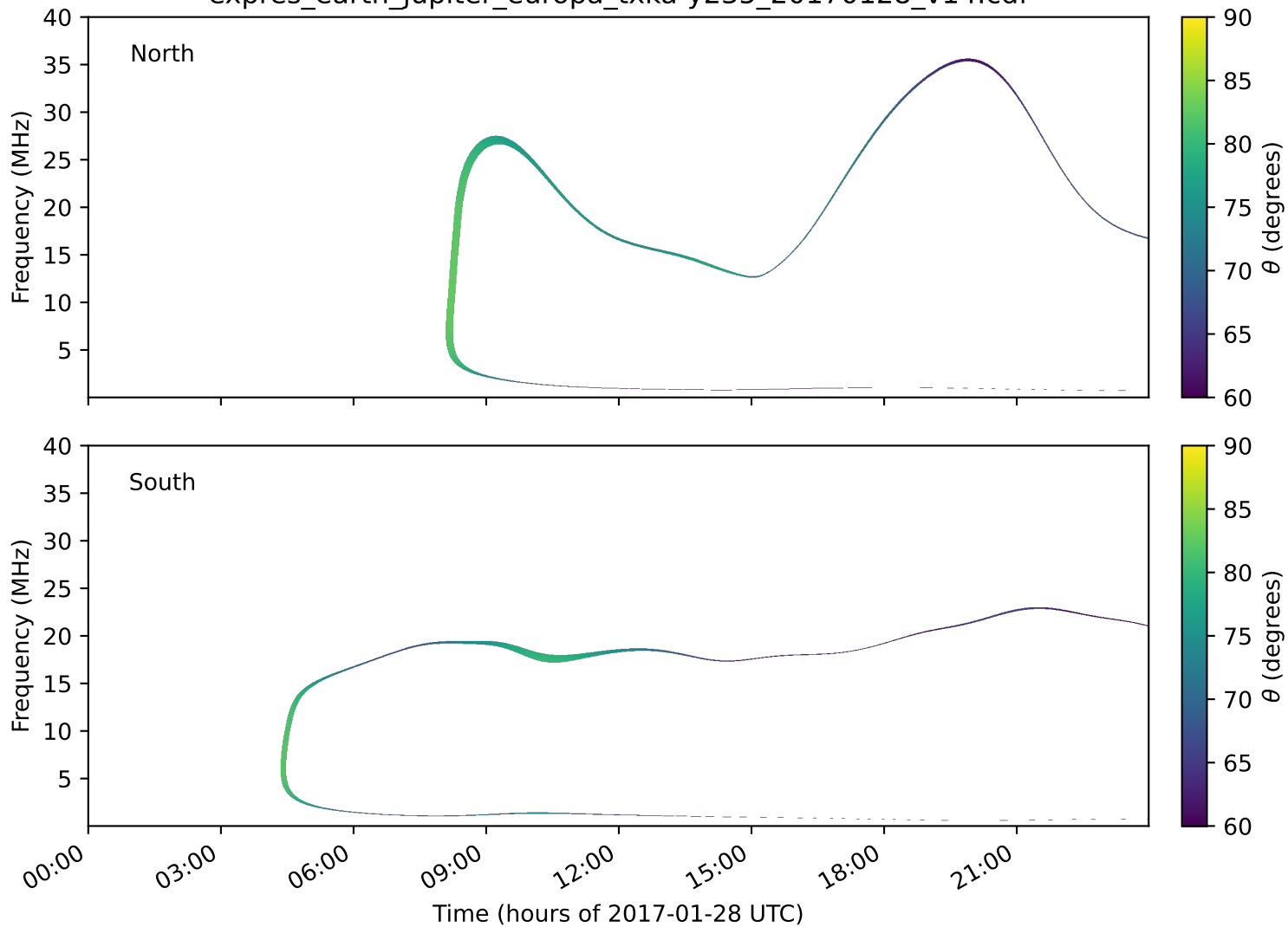
expres_earth_jupiter_europa_txka-y235_20170128_v14.cdf
