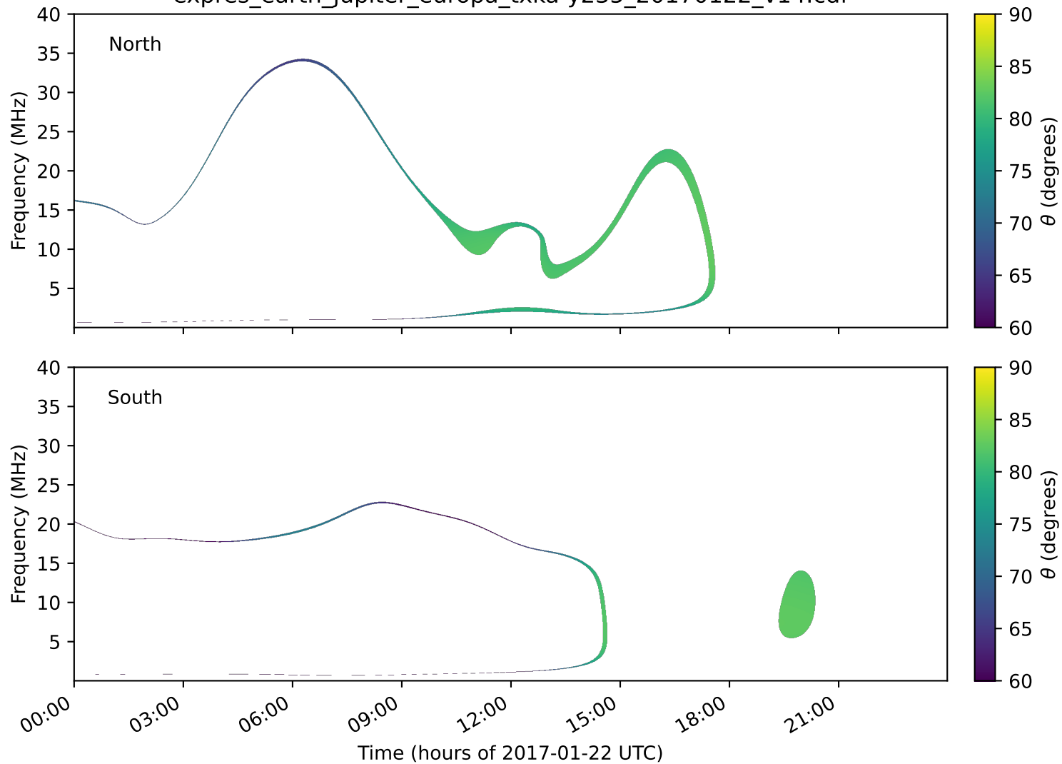
expres_earth_jupiter_europa_txka-y235_20170122_v14.cdf
