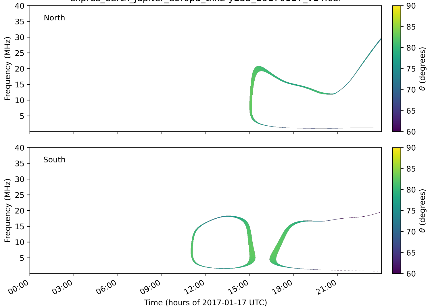
expres_earth_jupiter_europa_txka-y235_20170117_v14.cdf
