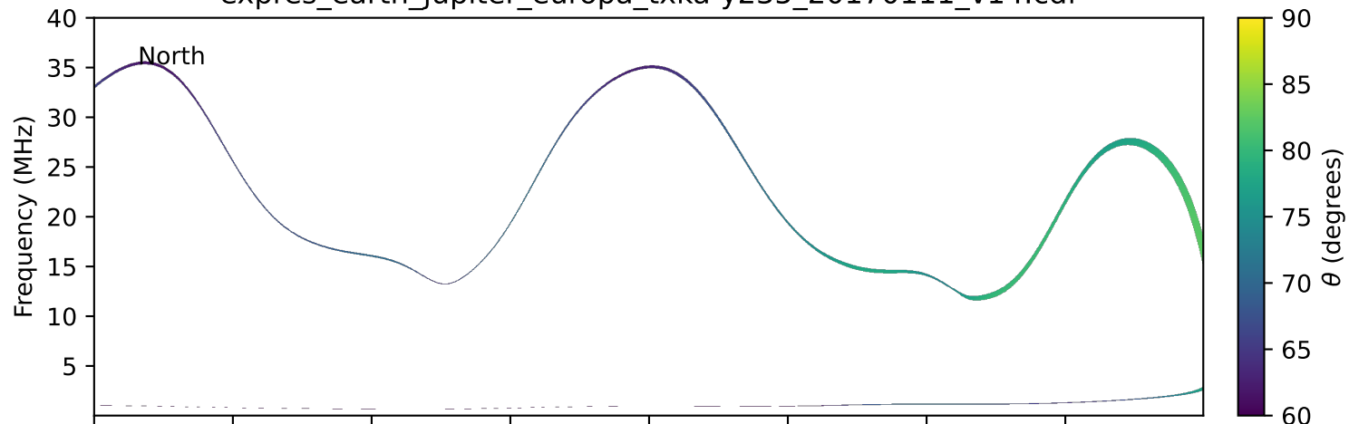
expres_earth_jupiter_europa_txka-y235_20170111_v14.cdf
