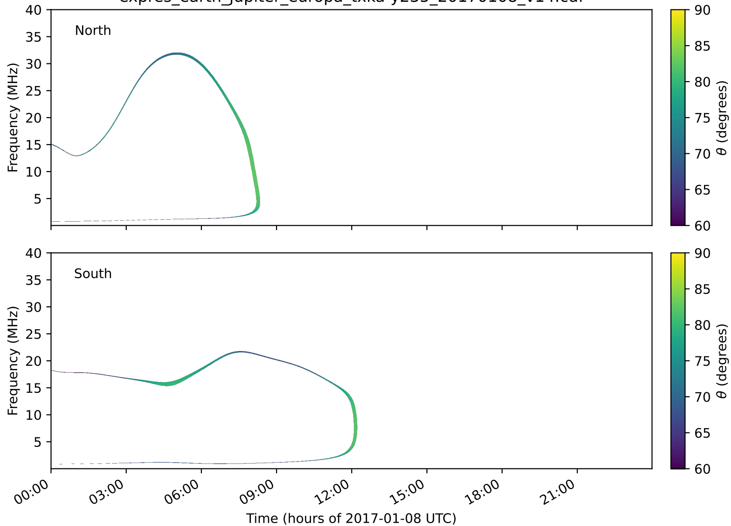
expres_earth_jupiter_europa_txka-y235_20170108_v14.cdf
