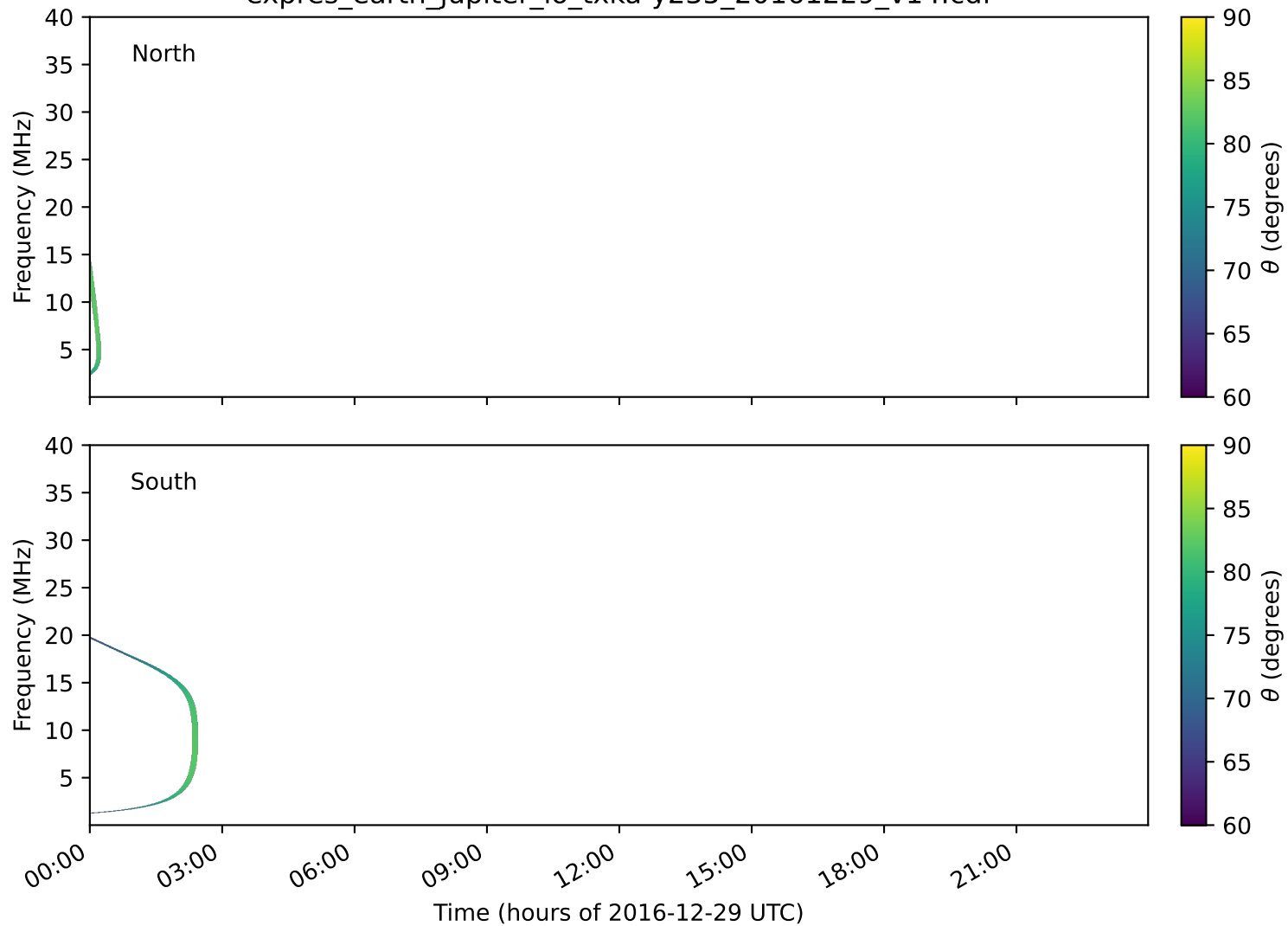
expres_earth_jupiter_io_txka-y235_20161229_v14.cdf
