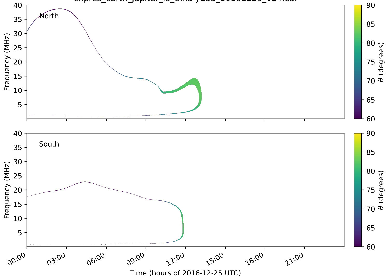
expres_earth_jupiter_io_txka-y235_20161225_v14.cdf
