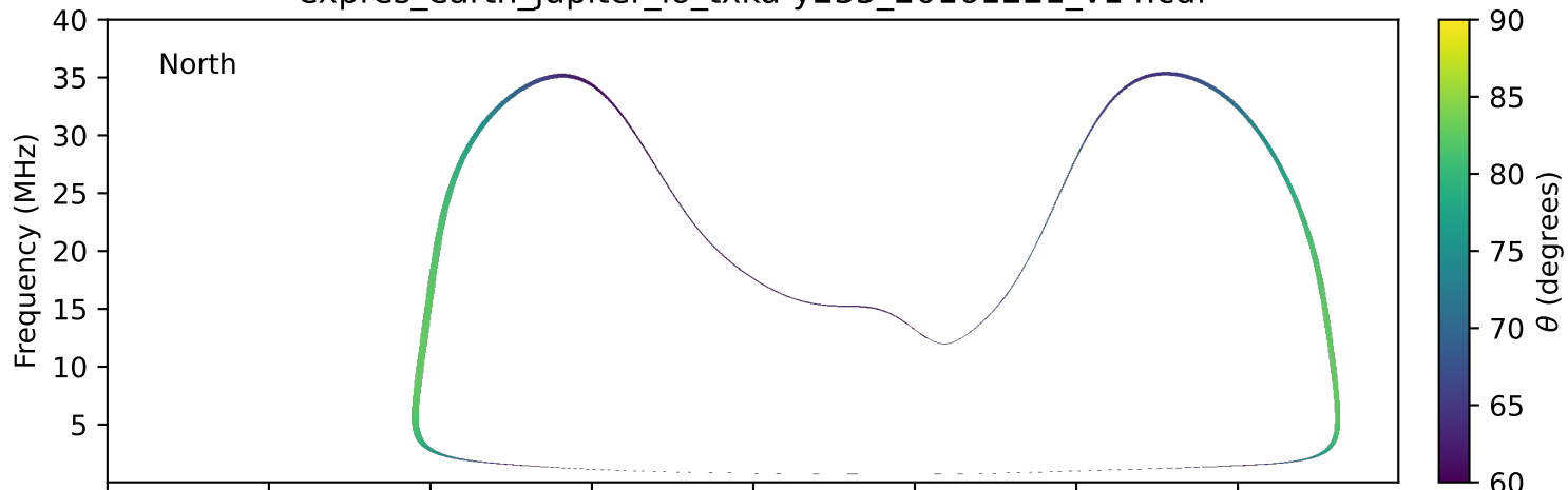
expres_earth_jupiter_io_txka-y235_20161221_v14.cdf
