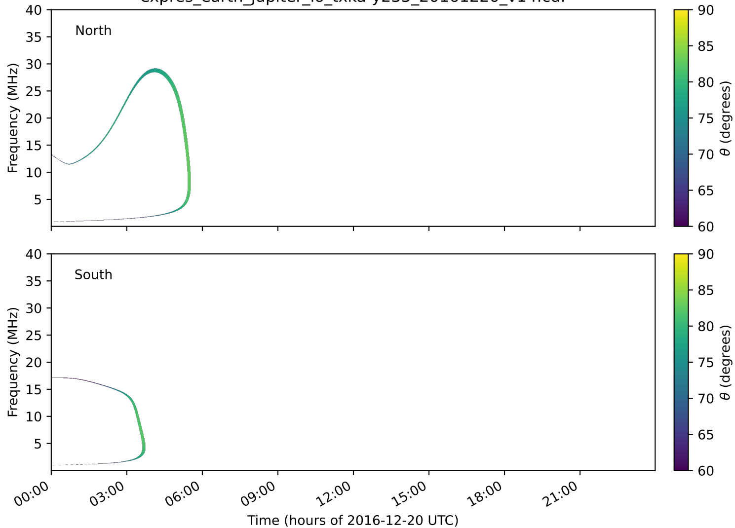
expres_earth_jupiter_io_txka-y235_20161220_v14.cdf
